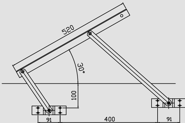
OE-BLU-FN-HD 520MM BLACK
