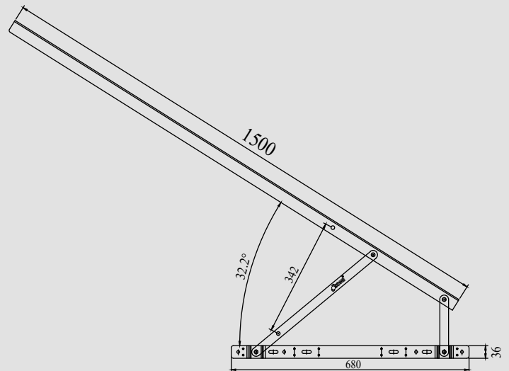
OE-BLU-FN-HD 1500MM BLACK
