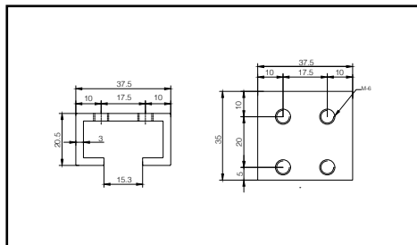
• Wall Bracket for Stabilizing Support Profile • Material: Aluminium. • Finish: BM & AN • Other Finish can also be available on request.
